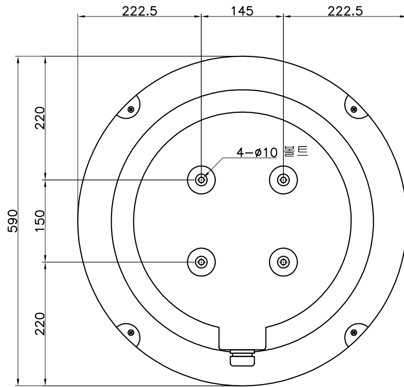
BOTTOM VIEW
