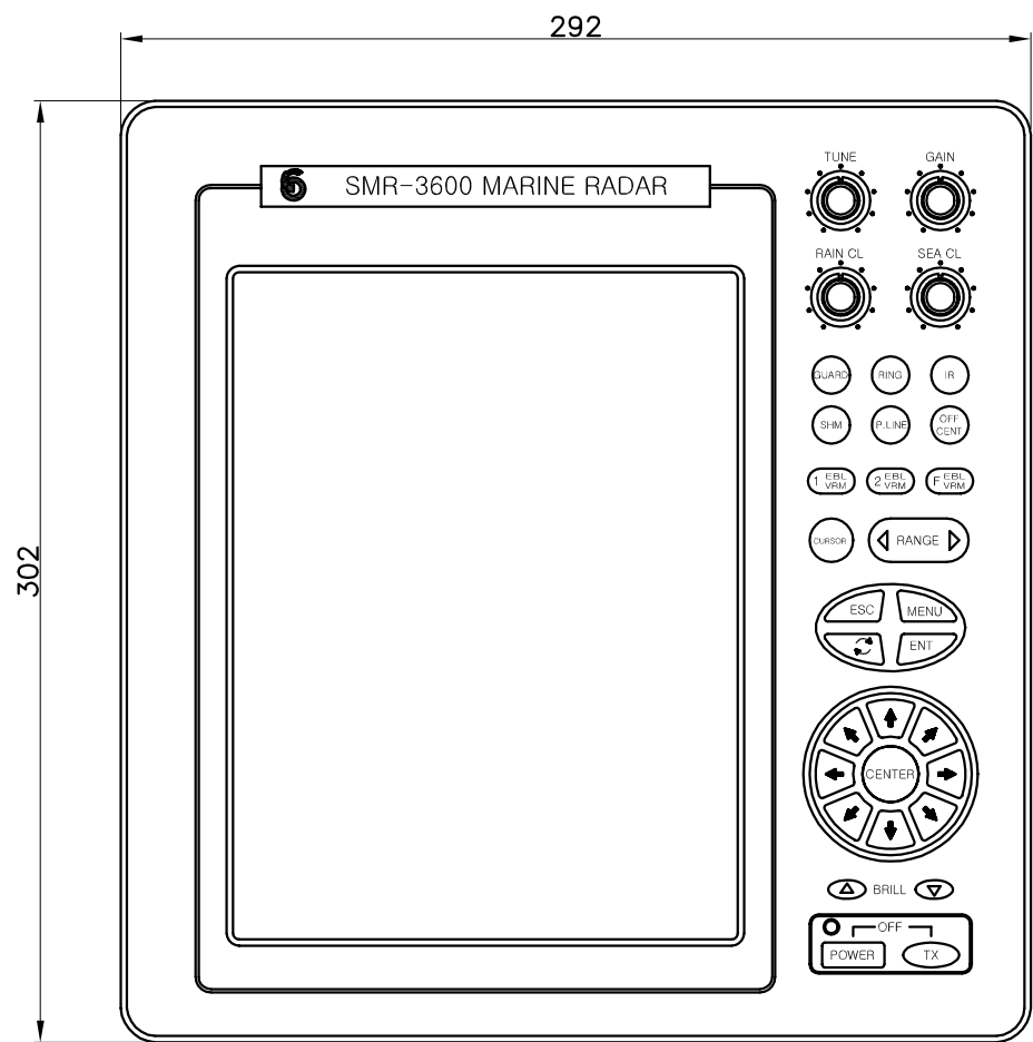
FRONT VIEW
