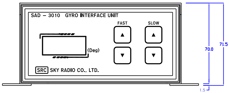
Outline Drawing of SAD - 3010 GYRO INTERFACE UNIT
